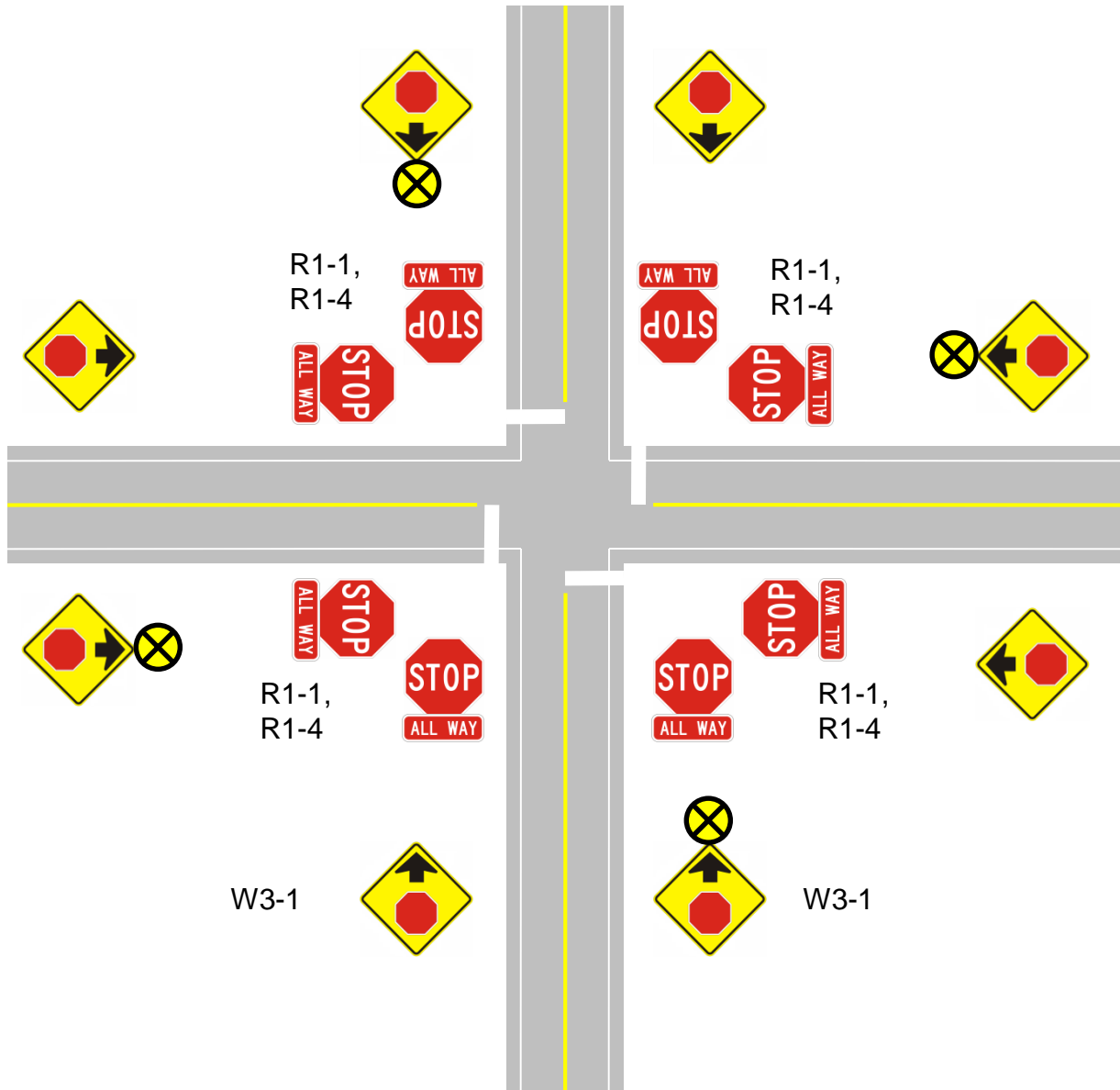
Type "B" Intersection Standard Package for 4-Way Stop Controlled Intersections
