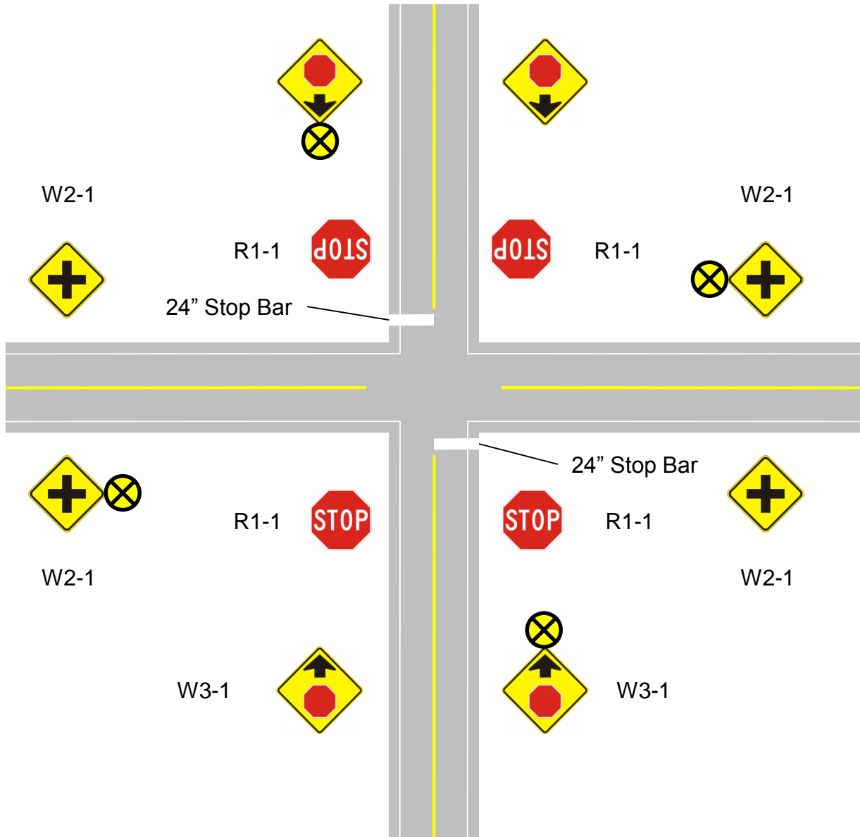
Type "C" Intersection Standard Package for 2-Way Stop Controlled Intersections
