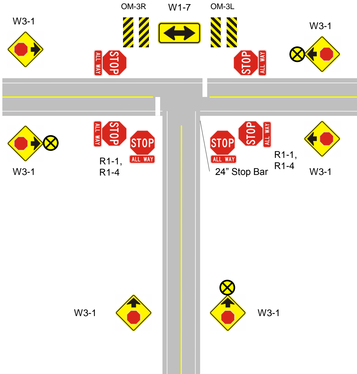
Type "D" Intersection Standard Package for T-Intersections with Three-Way Stop
