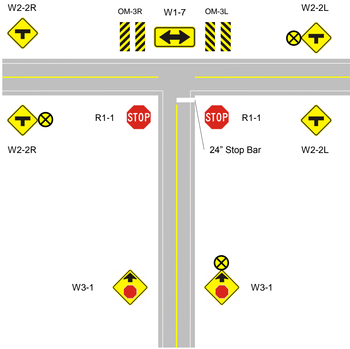
Type "A" Intersection Standard Package for T-Intersections with One Stop
