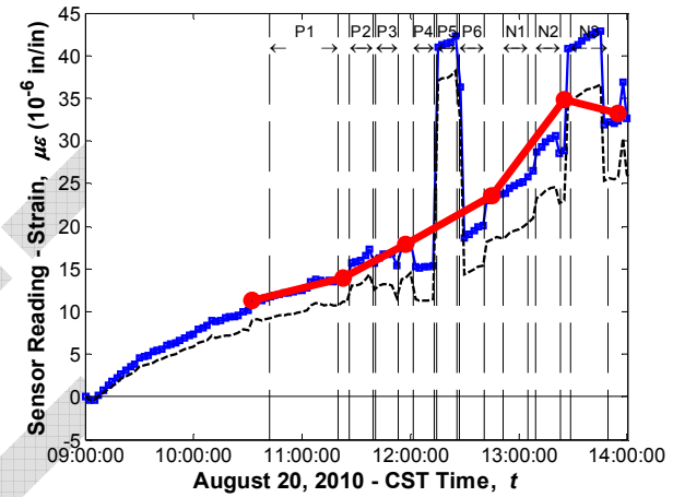
Sensor No. 72, Location Midspan (Vibrating wire gauge)
