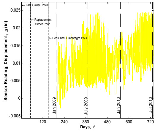
Sensor No. 58, Location G3, End Connection (Displacement meter)
