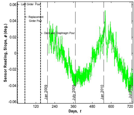
Sensor No. 56, Location G3S23, Support (Tiltmeter)
