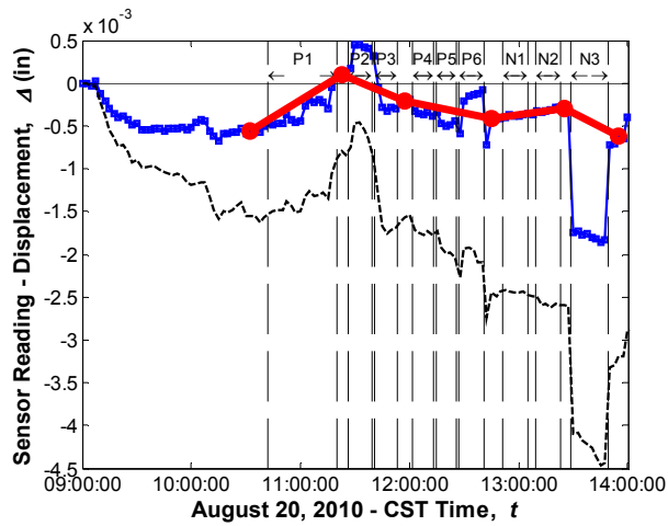
Sensor No. 9, Location G1, End Connection (Displacement meter)
