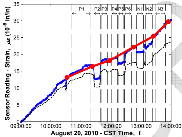
Sensor No. 65, Location G5S24, Midspan Top (Vibrating wire gauge)
