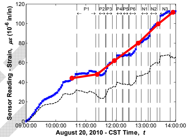
Sensor No. 6, Location G2S24, Support Top (Strandmeter)
