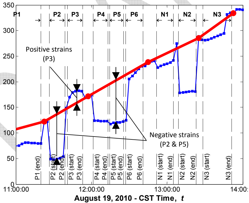
Figure 41 Strains in hairpin bars showing positive values for faraway load cases
