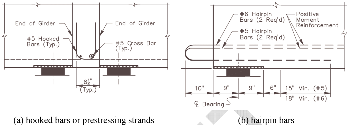
Figure 4 Alternatives for positive moment reinforcement (I)
