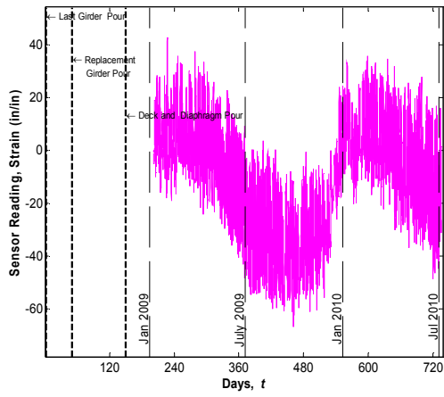
Sensor No. 82, Location G3S24, Midspan Middle (Vibrating wire gauge)
