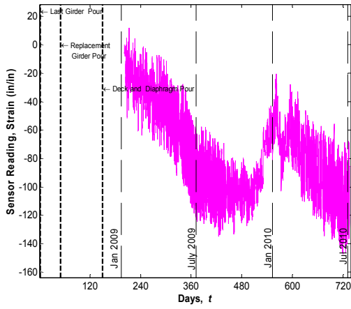
Sensor No. 84, Location G4S24, Midspan Top (Vibrating wire gauge)
