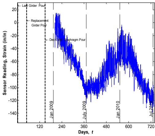
Sensor No. 70, Location G5S24, Midspan Deck (Sisterbar)
