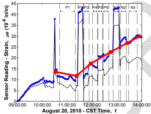
Sensor No. 69, Location G5S24, Midspan Bottom (Sisterbar)
