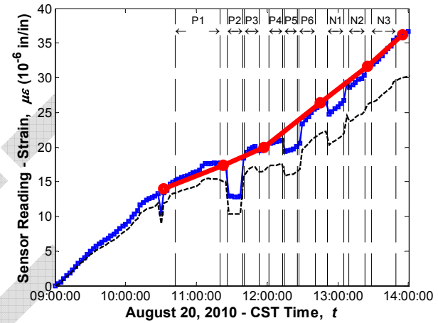
Sensor No. 68, Location G5S24, Midspan Top (Sisterbar)
