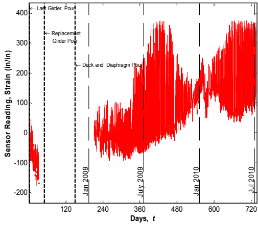
Sensor No. 49, Location G3S24, Support Bottom (Strandmeter)
