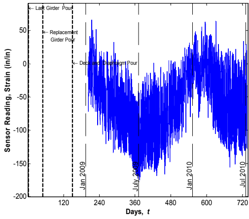
Sensor No. 5, Location G1S24, Support Top (Sisterbar)
