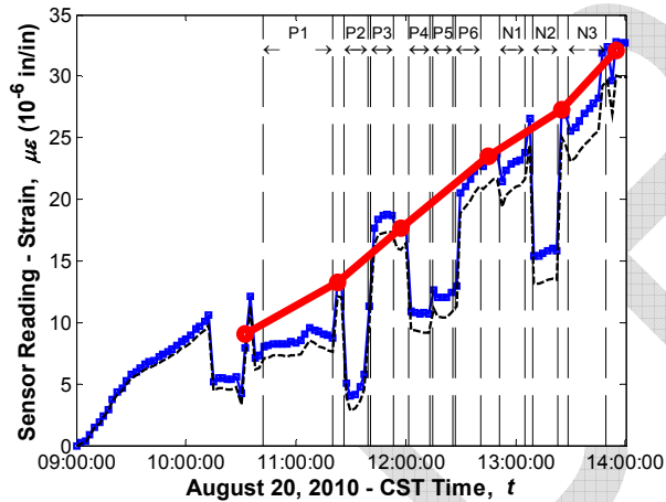
Sensor No. 44, Location G3S23, Support Bottom (Vibrating wire gauge)
