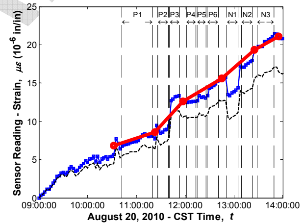
Sensor No. 33, Location G5S24, Support Top (Vibrating wire gauge)
