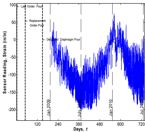
Sensor No. 53, Location G3S24, Support Top (Sisterbar)
