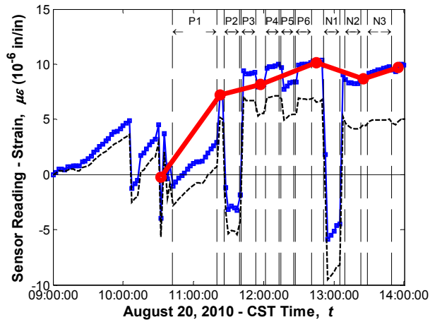
Sensor No. 38, Location G5S23, Support Bottom (Vibrating wire gauge)
