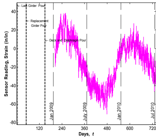
Sensor No. 36, Location G5S23, Support Top (Vibrating wire gauge)
