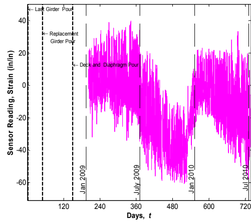
Sensor No. 83, Location G3S24, Midspan Bottom (Vibrating wire gauge)
