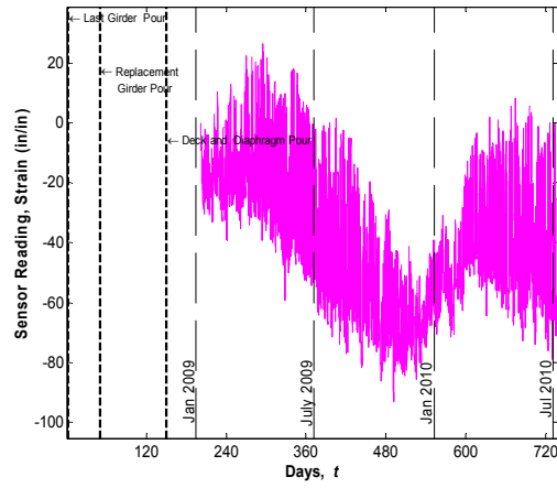
Sensor No. 44, Location G3S23, Support Bottom (Vibrating wire gauge)
