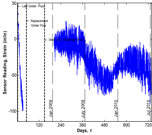
Sensor No. 94, Location G4S24, Midspan Bottom (Sisterbar)
