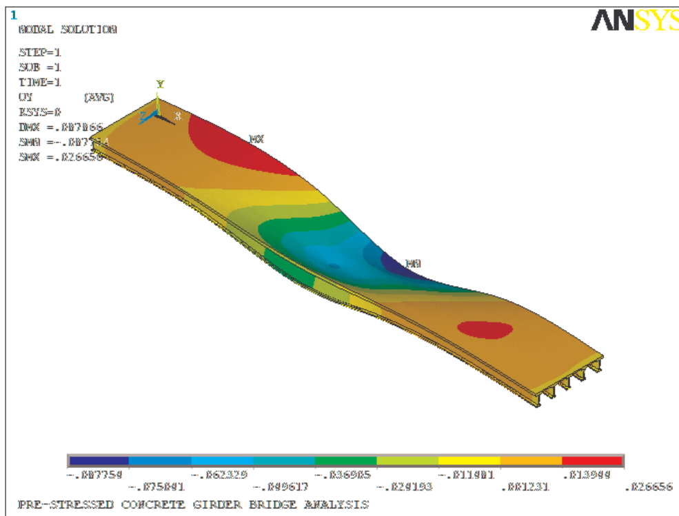
Figure 40 Contours of vertical displacement (Case P5).
