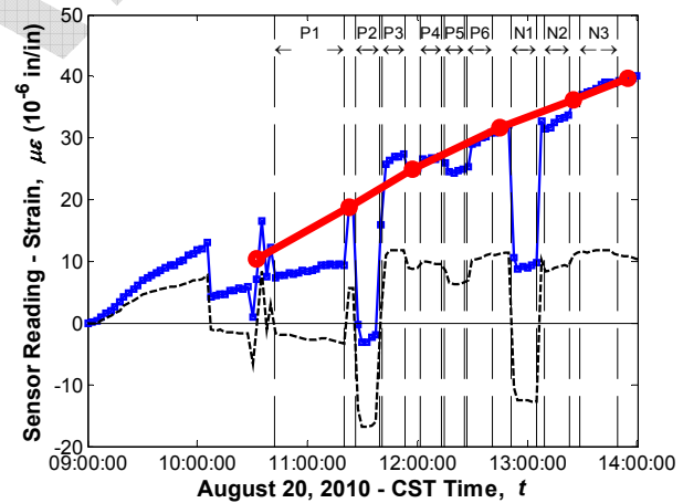
Sensor No. 45, Location G5S24, Support Bottom (Strandmeter)
