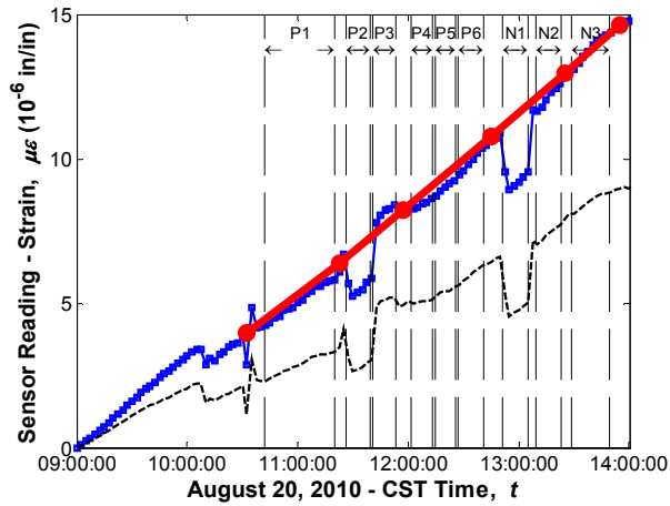
Sensor No. 34, Location G5S24, Support Middle (Vibrating wire gauge)
