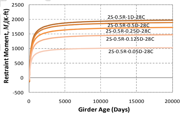
(c) L_1 = 0.5 \cdot L_2 and Age = 28 days
