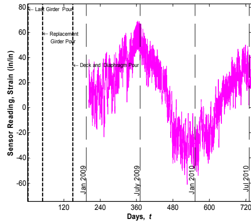
Sensor No. 38, Location G5S23, Support Bottom (Vibrating wire gauge)
