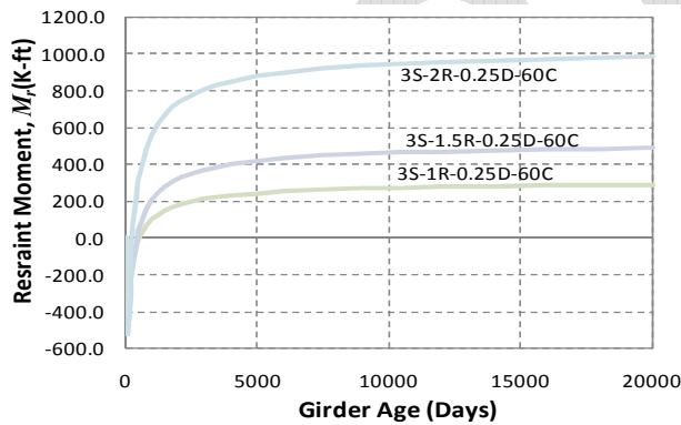
(c) Age = 60 days and I_{dia} = 0.25 \cdot I_g
