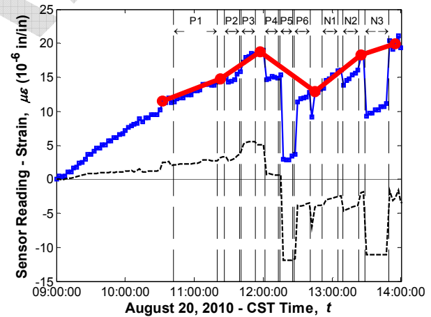
Sensor No. 4, Location G1S23, Support Bottom (Strandmeter)
