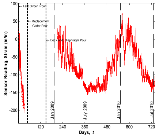
Sensor No. 89, Location G3S24, Midspan Bottom (Strandmeter)
