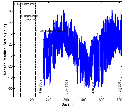
Sensor No. 69, Location G5S24, Midspan Bottom (Sisterbar)
