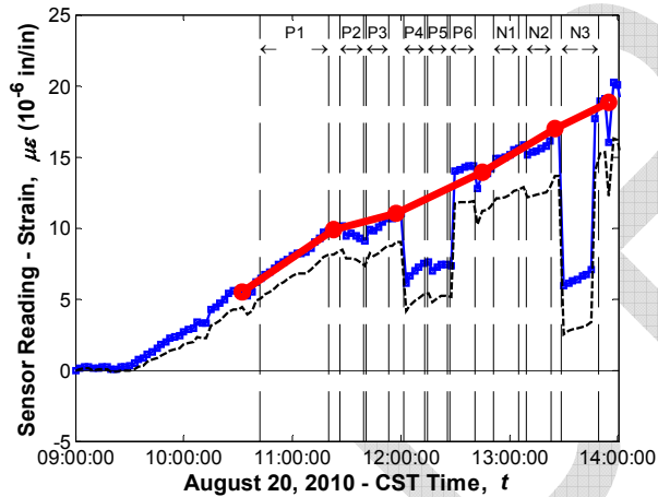
Sensor No. 22, Location G1S23, Support Bottom (Vibrating wire gauge)
