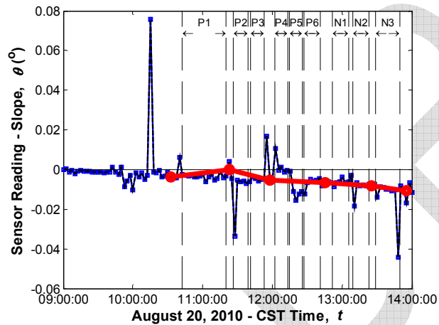
Sensor No. 7, Location G1S24, Support (Tiltmeter)
