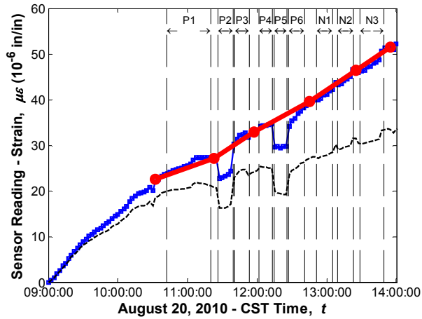
Sensor No. 87, Location G4S24, Midspan Top (Strandmeter)
