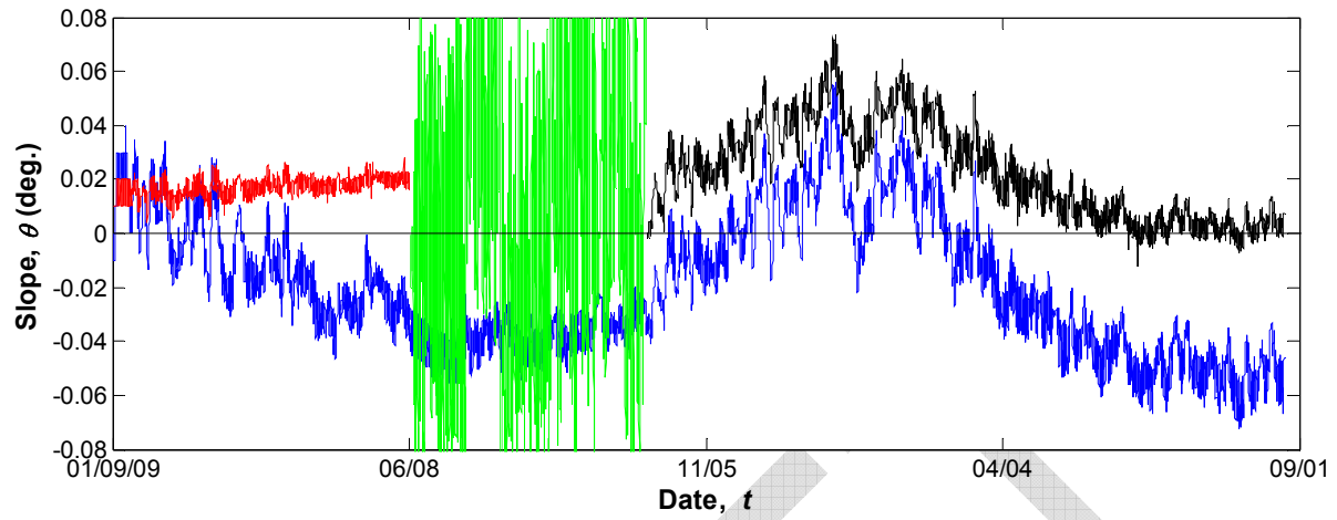
Figure 14 Joined data record for tiltmeter (TM) at G1 in Spans 23 and 24.
