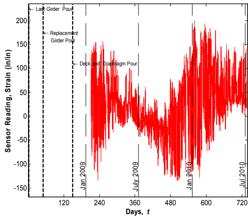
Sensor No. 45, Location G5S24, Support Bottom (Strandmeter)
