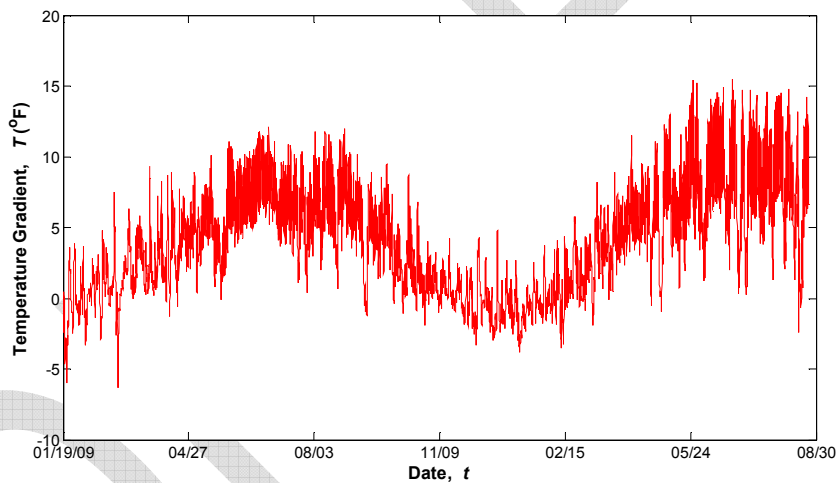
Figure 30 Temperature gradient (Girder G3 in the middle of Span 24).
