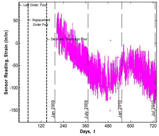
Sensor No. 19, Location G1S24, Support Bottom (Vibrating wire gauge)
