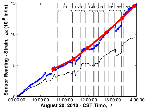
Sensor No. 42, Location G3S23, Support Top (Vibrating wire gauge)
