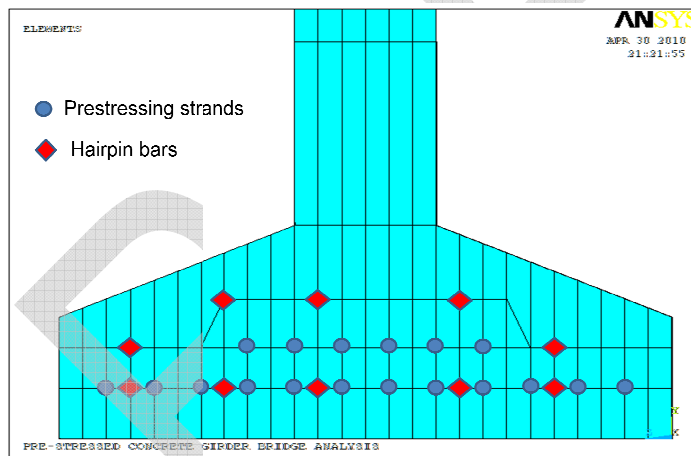
(b) Bottom flange showing reinforcement
