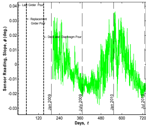
Sensor No. 57, Location G5S23, Support (Tiltmeter)
