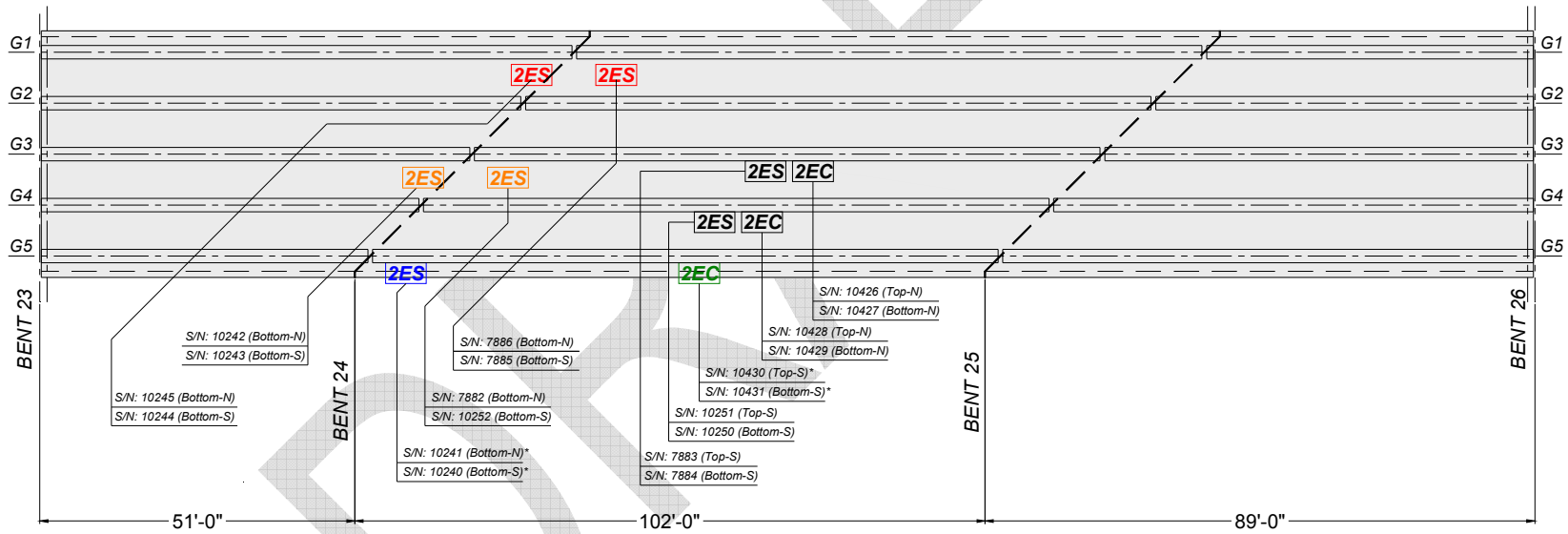
Figure A-15 Distribution of sensors on system multiplexers.
