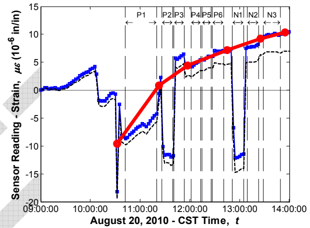
Sensor No. 35, Location G5S24, Support Bottom (Vibrating wire gauge)
