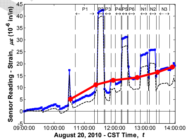
Sensor No. 86, Location G4S24, Midspan Bottom (Vibrating wire gauge)
