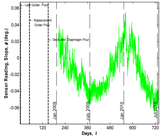
Sensor No. 8, Location G1S23, Support (Tiltmeter)
