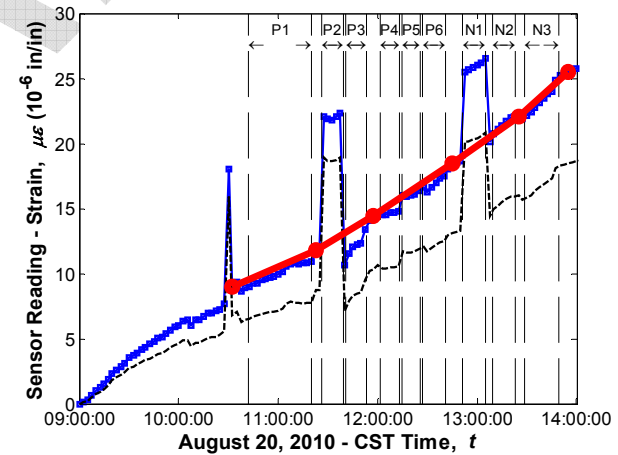
Sensor No. 66, Location G5S24, Midspan Middle (Vibrating wire gauge)
