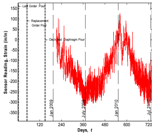
Sensor No. 48, Location G4S24, Support Top (Strandmeter)
