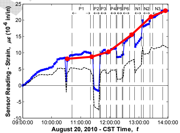
Sensor No. 70, Location G5S24, Midspan Deck (Sisterbar)
