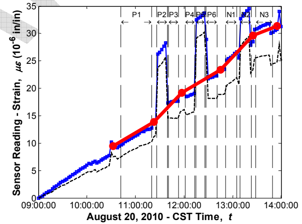
Sensor No. 82, Location G3S24, Midspan Middle (Vibrating wire gauge)
