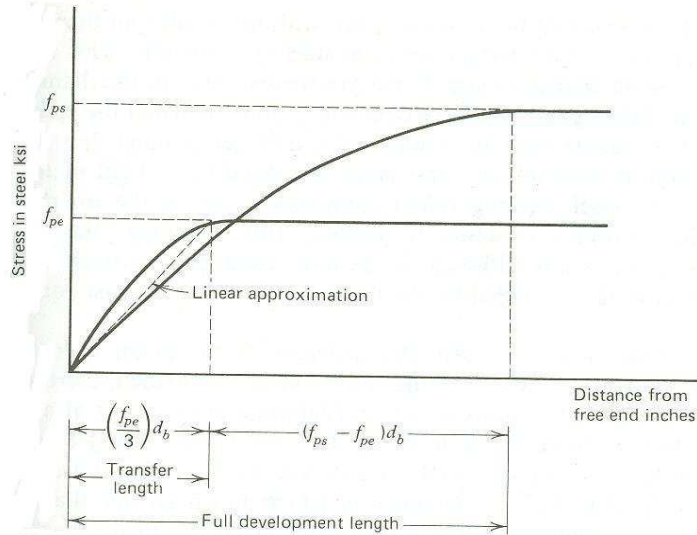
Figure 16 Transfer length model used in estimating M_{cr} at girder ends (Nilson 1987)
