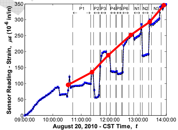
Sensor No. 49, Location G3S24, Support Bottom (Strandmeter)
