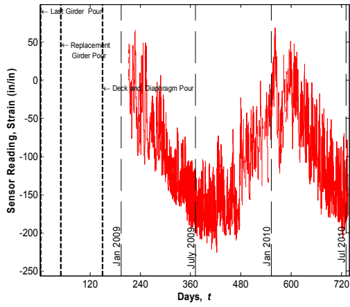
Sensor No. 1, Location G1S24, Support Bottom (Strandmeter)
