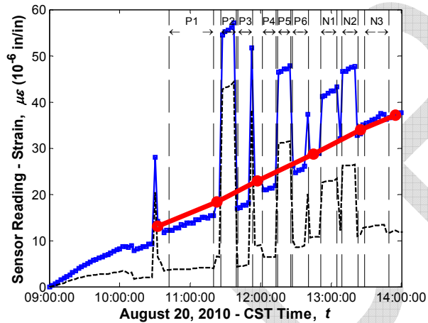
Sensor No. 89, Location G3S24, Midspan Bottom (Strandmeter)
