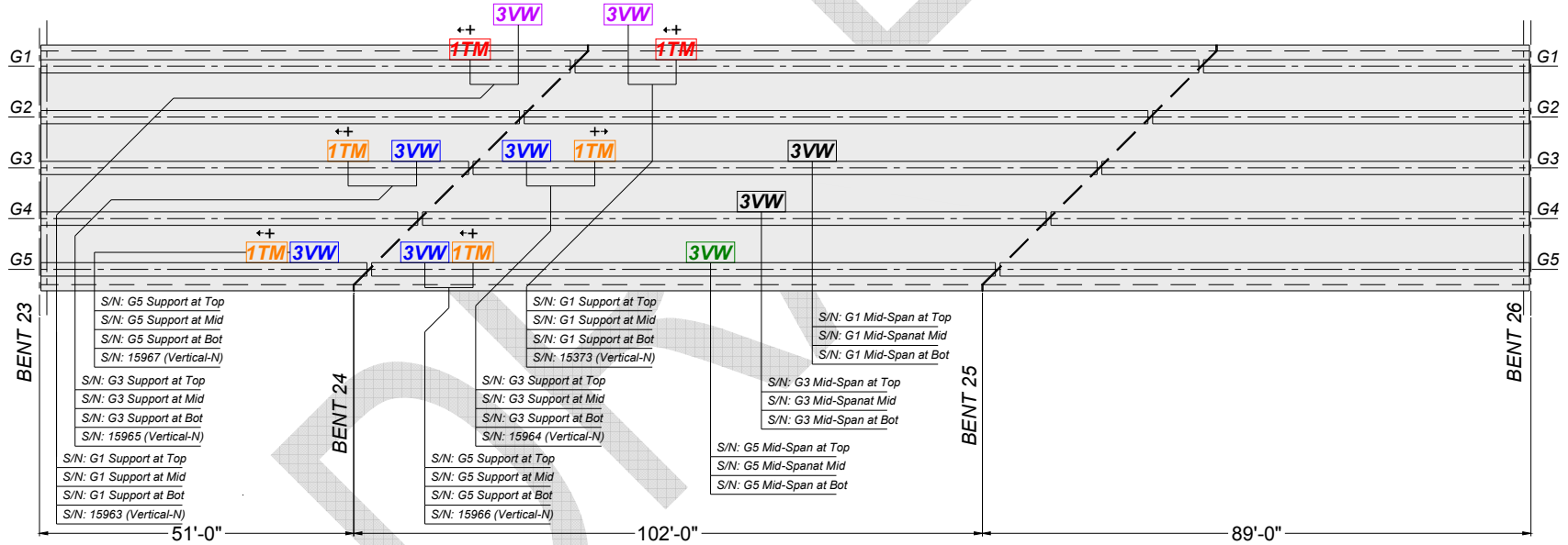
Figure A-17 Distribution of sensors on system multiplexers.
