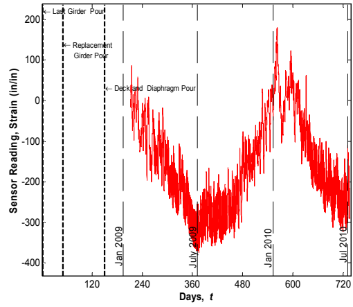
Sensor No. 6, Location G2S24, Support Top (Strandmeter)
