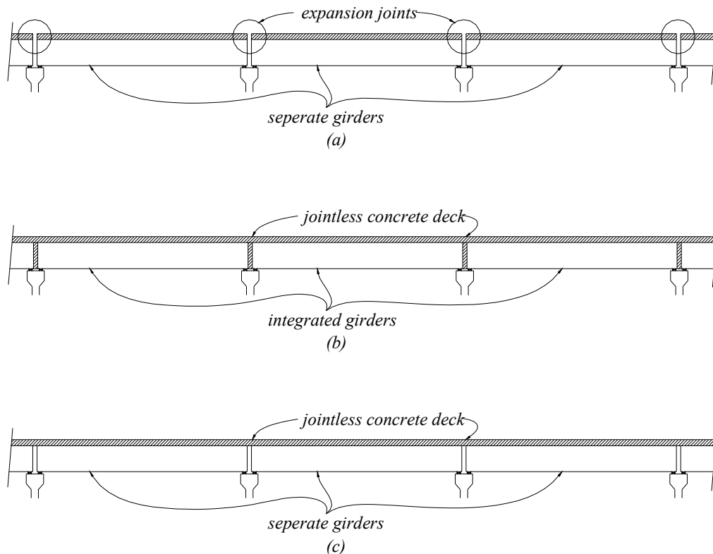
Figure 1 Typical continuity conditions in precast PSC girder bridges: (a) simply-supported, (b) fully continuous, (c) partially continuous. (2)
