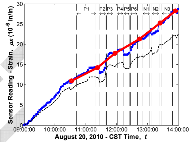
Sensor No. 84, Location G4S24, Midspan Top (Vibrating wire gauge)
