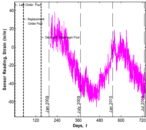
Sensor No. 39, Location G3S24, Support Top (Vibrating wire gauge)
