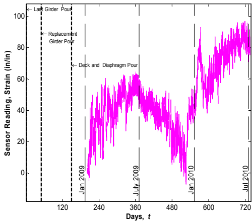
Sensor No. 37, Location G5S23, Support Middle (Vibrating wire gauge)
