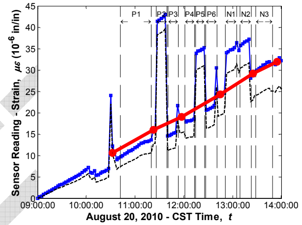
Sensor No. 92, Location G3S24, Midspan Bottom (Sisterbar)
