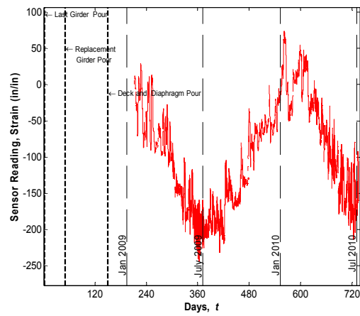
Sensor No. 4, Location G1S23, Support Bottom (Strandmeter)
