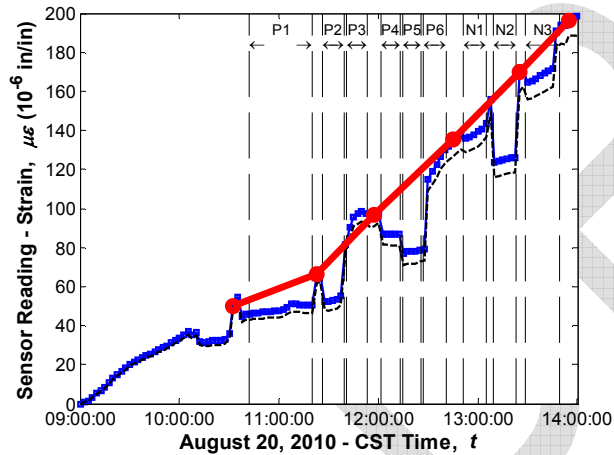
Sensor No. 52, Location G3S24, Support Bottom (Strandmeter)
