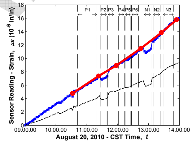
Sensor No. 37, Location G5S23, Support Middle (Vibrating wire gauge)
