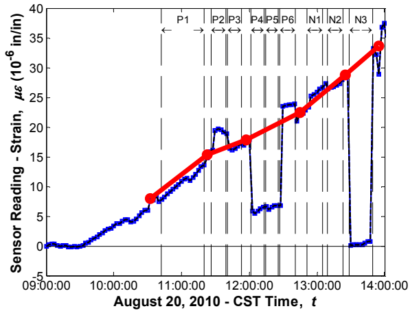
Sensor No. 1, Location G1S24, Support Bottom (Strandmeter)
