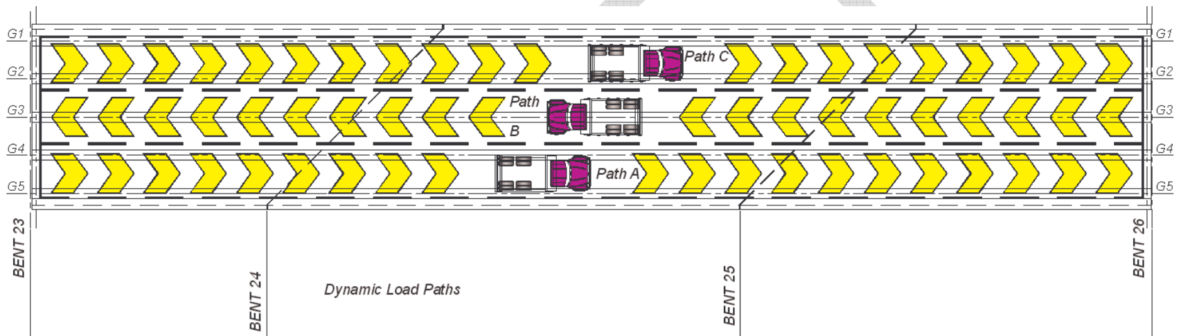
Figure 25 Truck paths for the dynamic load tests.
