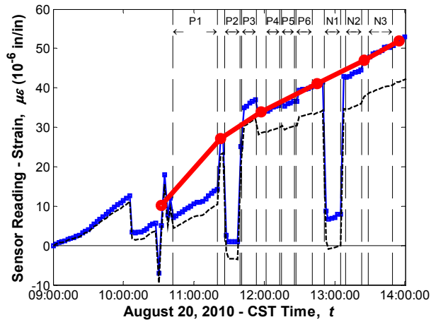
Sensor No. 46, Location G5S24, Support Bottom (Strandmeter)
