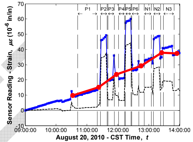
Sensor No. 88, Location G4S24, Midspan Bottom (Strandmeter)
