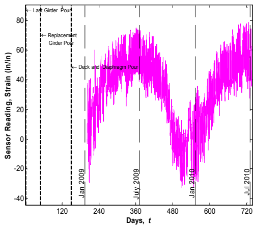
Sensor No. 66, Location G5S24, Midspan Middle (Vibrating wire gauge)
