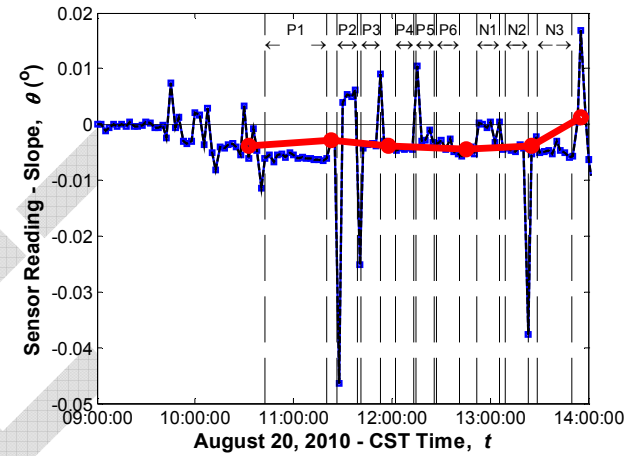
Sensor No. 60, Location G5S24, Support (Tiltmeter)
