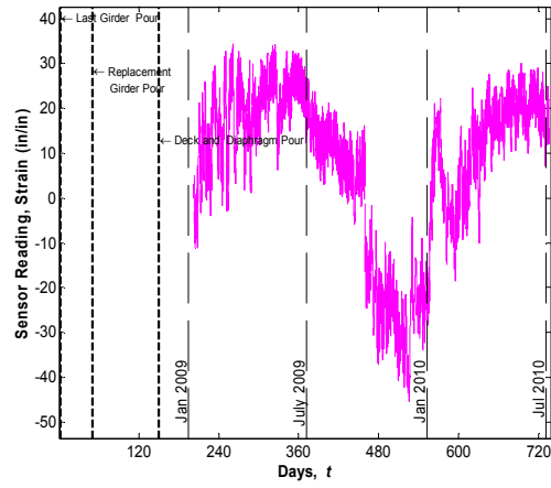
Sensor No. 34, Location G5S24, Support Middle (Vibrating wire gauge)
