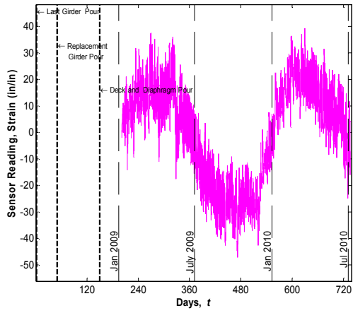
Sensor No. 18, Location G1S24, Support Middle (Vibrating wire gauge)
