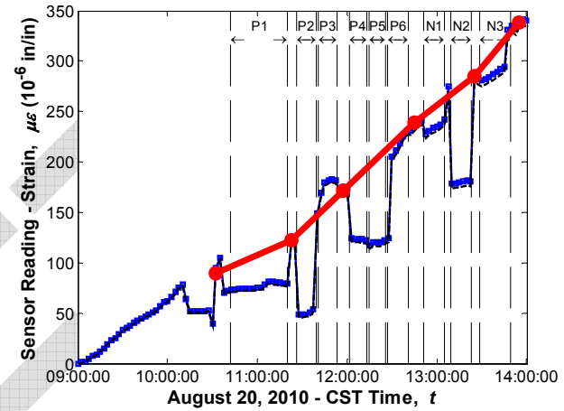
Sensor No. 51, Location G3S23, Support Bottom (Strandmeter)
