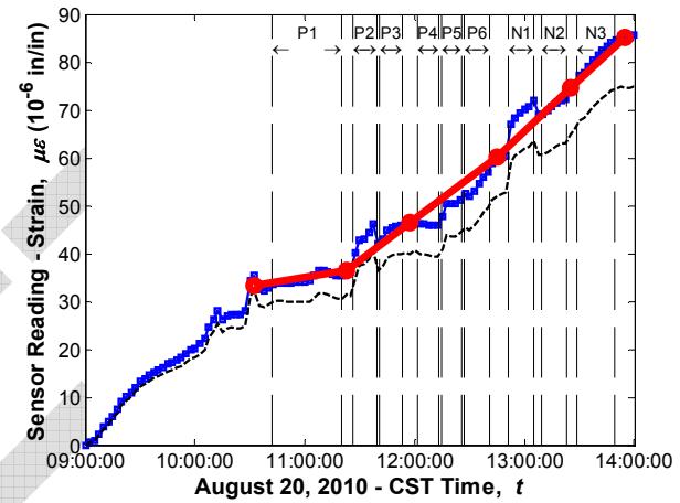
Sensor No. 47, Location G5S24, Support Top (Sisterbar)
