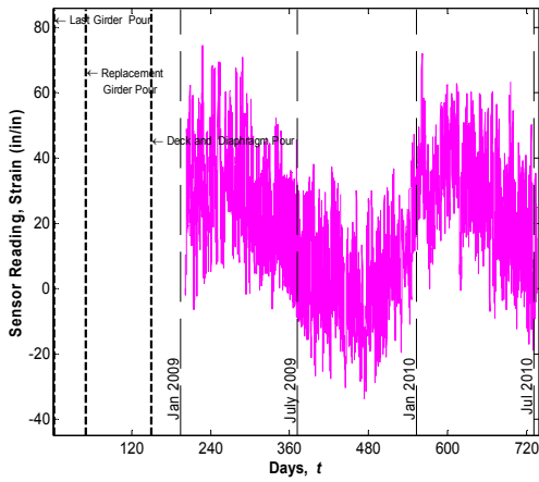
Sensor No. 86, Location G4S24, Midspan Bottom (Vibrating wire gauge)
