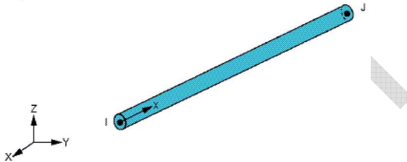
Figure E-2 Geometry, node location and co-ordinate system for LINK68.
