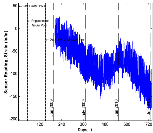
Sensor No. 93, Location G4S24, Midspan Top (Sisterbar)
