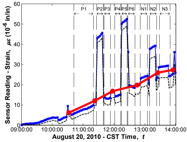
Sensor No. 83, Location G3S24, Midspan Bottom (Vibrating wire gauge)
