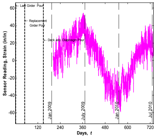
Sensor No. 35, Location G5S24, Support Bottom (Vibrating wire gauge)
