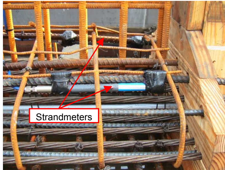
Figure A-1 Strandmeters installed on hairpin bars at girder ends.
