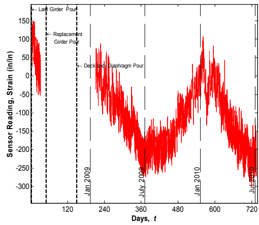
Sensor No. 87, Location G4S24, Midspan Top (Strandmeter)
