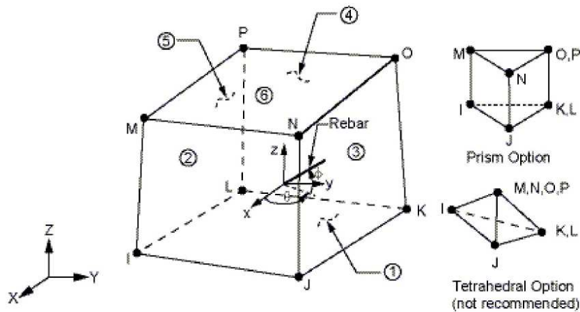
Figure E-3 Geometry, node location and co-ordinate system for SOLID65.
