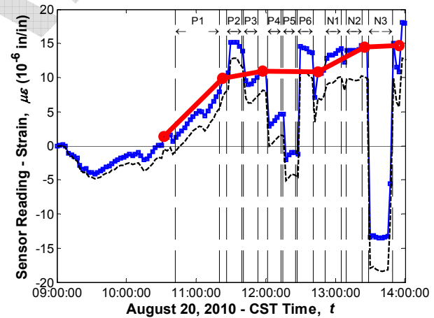
Sensor No. 19, Location G1S24, Support Bottom (Vibrating wire gauge)
