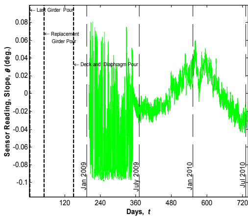
Sensor No. 54, Location G5S24, Support (Tiltmeter)
