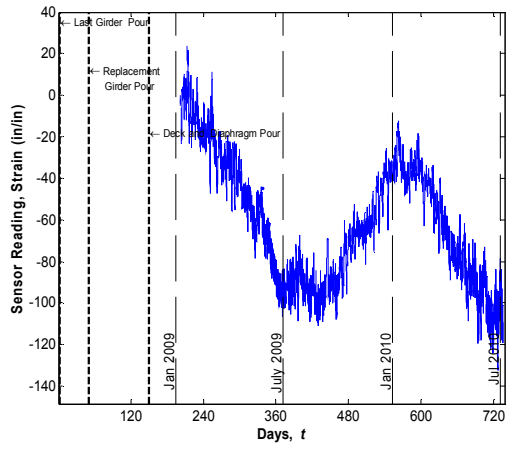
Sensor No. 96, Location G4S24, Midspan Deck (Sisterbar)
