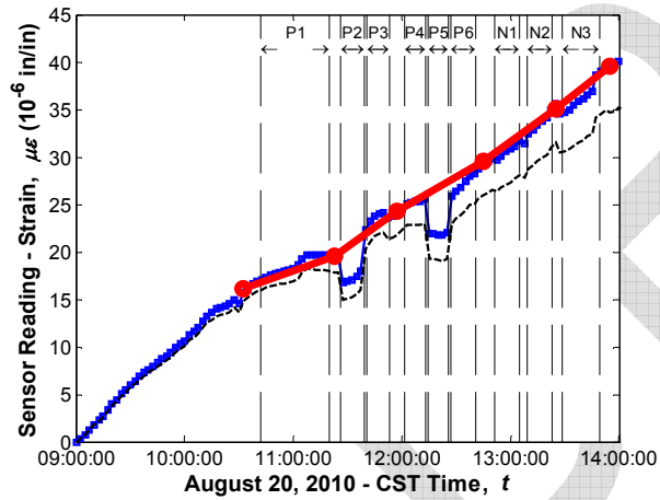
Sensor No. 93, Location G4S24, Midspan Top (Sisterbar)
