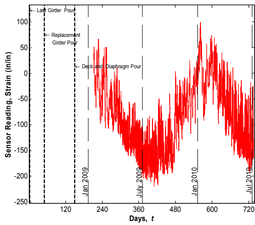
Sensor No. 3, Location G1S23, Support Bottom (Strandmeter)
