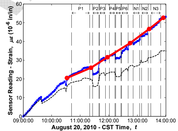
Sensor No. 90, Location G3S24, Midspan Top (Strandmeter)
