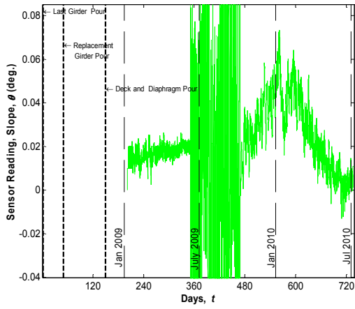
Sensor No. 7, Location G1S24, Support (Tiltmeter)
