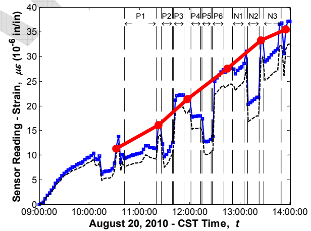
Sensor No. 41, Location G3S24, Support Bottom (Vibrating wire gauge)
