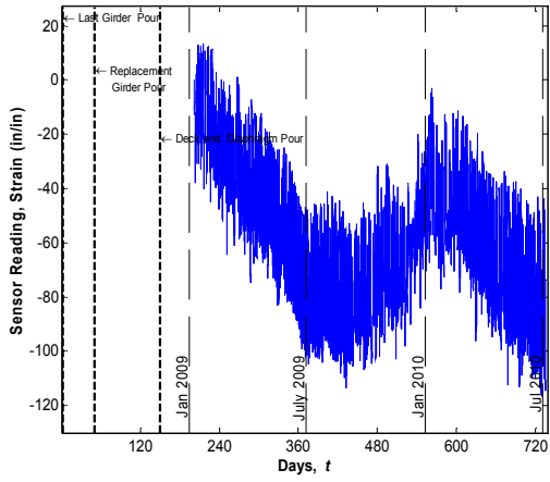
Sensor No. 68, Location G5S24, Midspan Top (Sisterbar)
