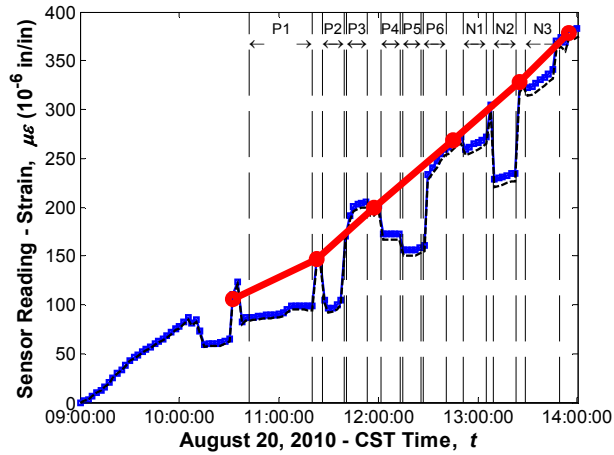
Sensor No. 50, Location G3S23, Support Bottom (Strandmeter)
