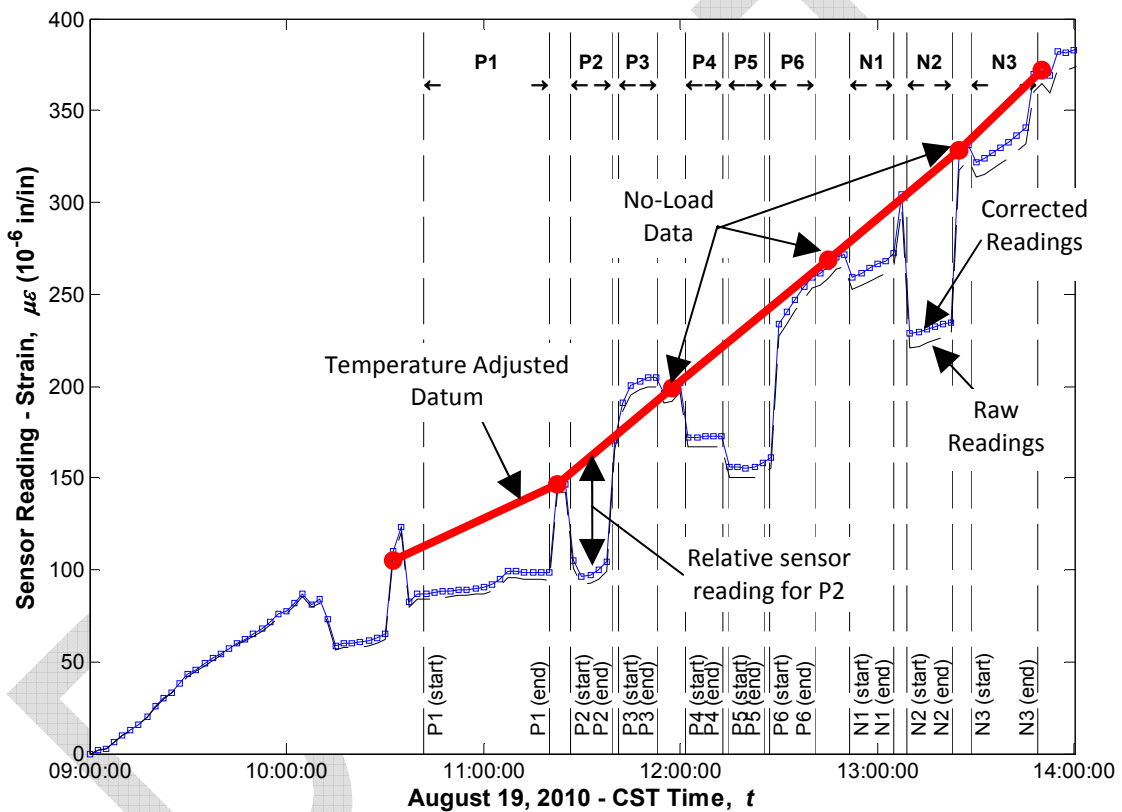
Figure 27 Sample sensor reading during static live load testing (Sensor #50 – G3, Span 23, hairpin bar).
