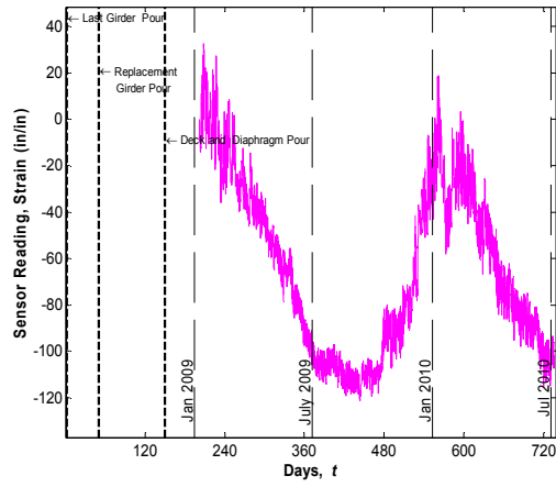
Sensor No. 40, Location G3S24, Support Middle (Vibrating wire gauge)
