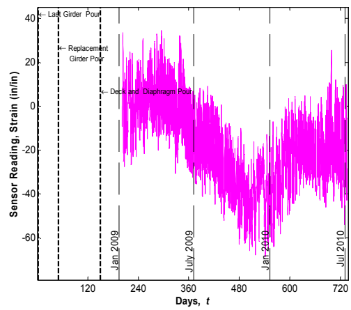
Sensor No. 67, Location G5S24, Midspan Bottom (Vibrating wire gauge)
