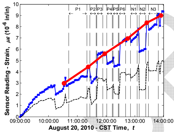
Sensor No. 40, Location G3S24, Support Middle (Vibrating wire gauge)
