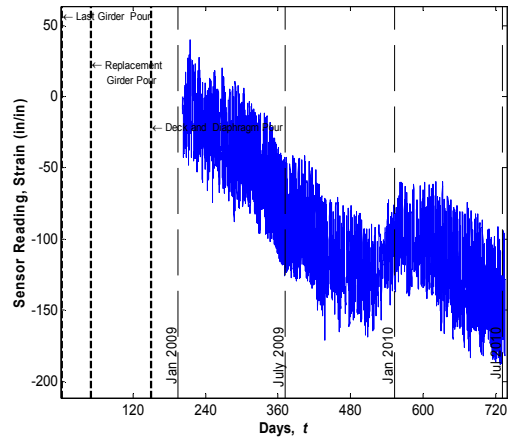
Sensor No. 91, Location G3S24, Midspan Top (Sisterbar)
