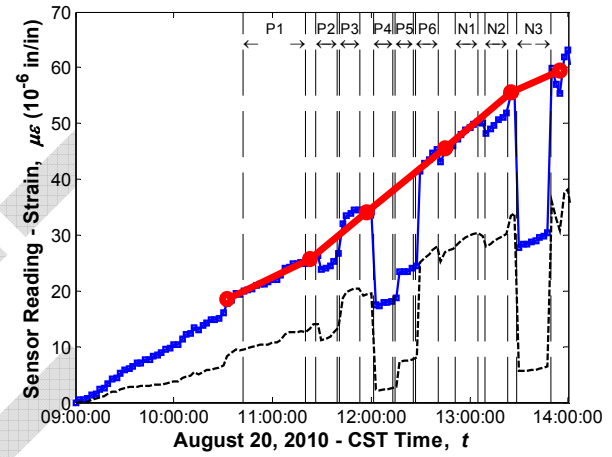
Sensor No. 2, Location G1S24, Support Bottom (Strandmeter)
