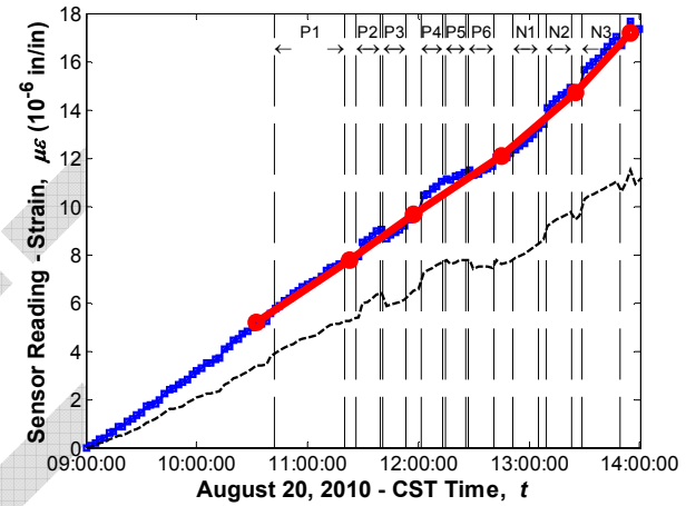
Sensor No. 17, Location G1S24, Support Top (Vibrating wire gauge)
