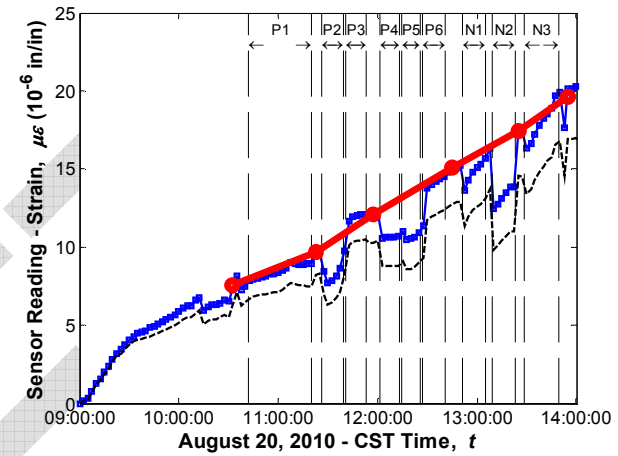
Sensor No. 43, Location G3S23, Support Middle (Vibrating wire gauge)
