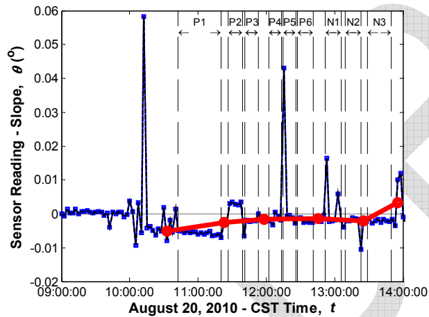
Sensor No. 57, Location G5S23, Support (Tiltmeter)
