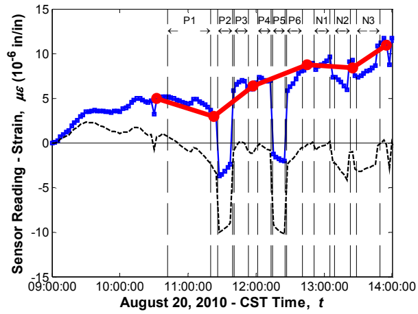
Sensor No. 95, Location G3S24, Midspan Deck (Sisterbar)
