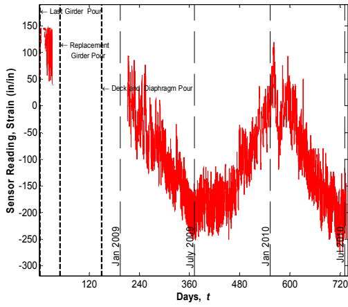
Sensor No. 90, Location G3S24, Midspan Top (Strandmeter)
