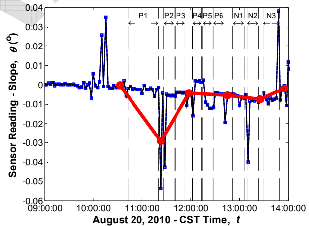
Sensor No. 8, Location G1S23, Support (Tiltmeter)
