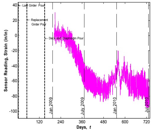
Sensor No. 81, Location G3S24, Midspan Top (Vibrating wire gauge)
