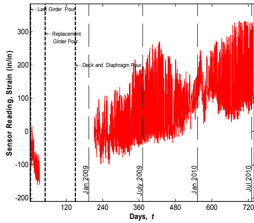
Sensor No. 52, Location G3S24, Support Bottom (Strandmeter)
