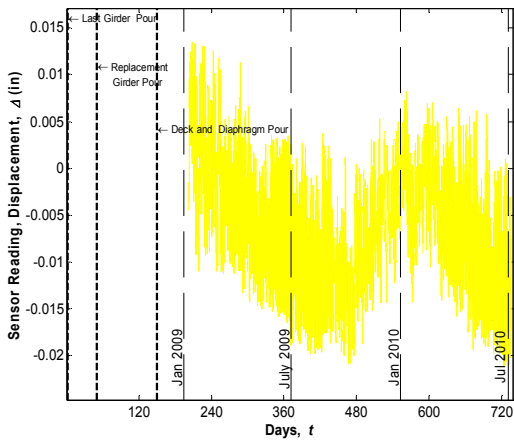
Sensor No. 9, Location G1, End Connection (Displacement meter)
