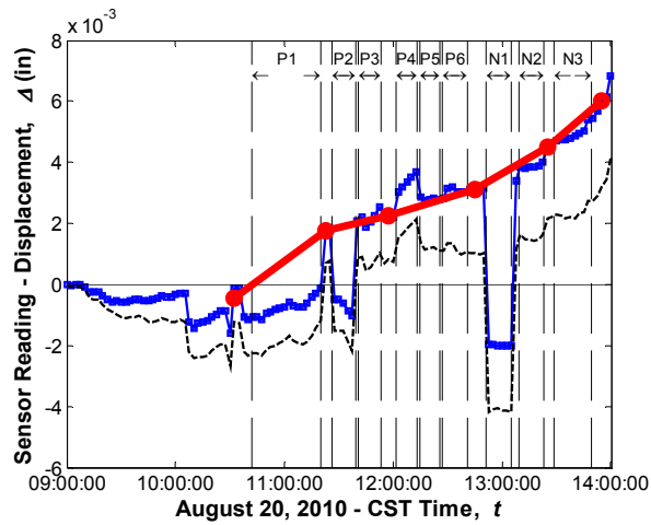
Sensor No. 59, Location G5, End Connection (Displacement meter)
