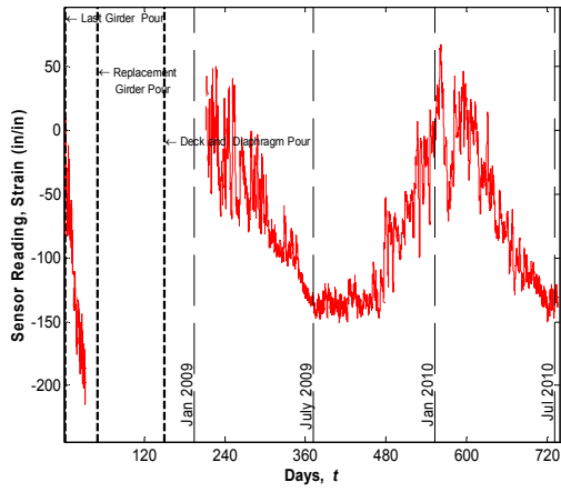
Sensor No. 88, Location G4S24, Midspan Bottom (Strandmeter)
