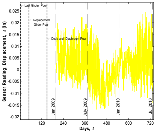
Sensor No. 59, Location G5, End Connection (Displacement meter)
