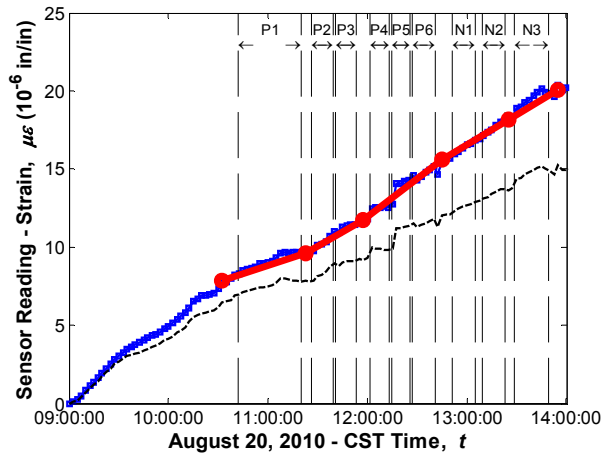
Sensor No. 20, Location G1S23, Support Top (Vibrating wire gauge)
