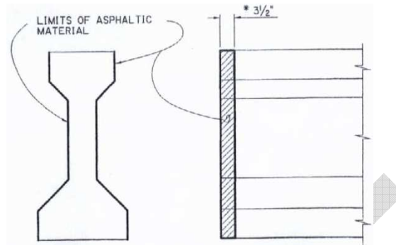
Figure 3 Bond breaker at girder ends
