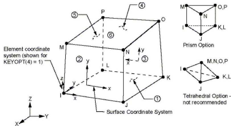
Figure E-5 Geometry, node location and co-ordinate system for SOLID45.
