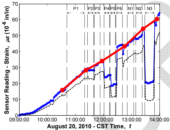
Sensor No. 3, Location G1S23, Support Bottom (Strandmeter)
