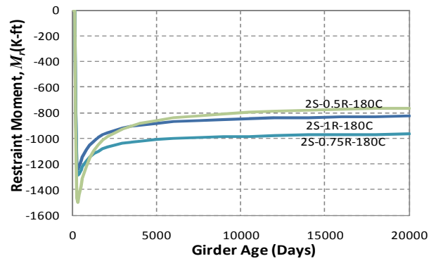
(a) Age = 180 days and I_{dia} = 0
