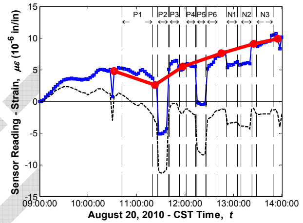
Sensor No. 96, Location G4S24, Midspan Deck (Sisterbar)
