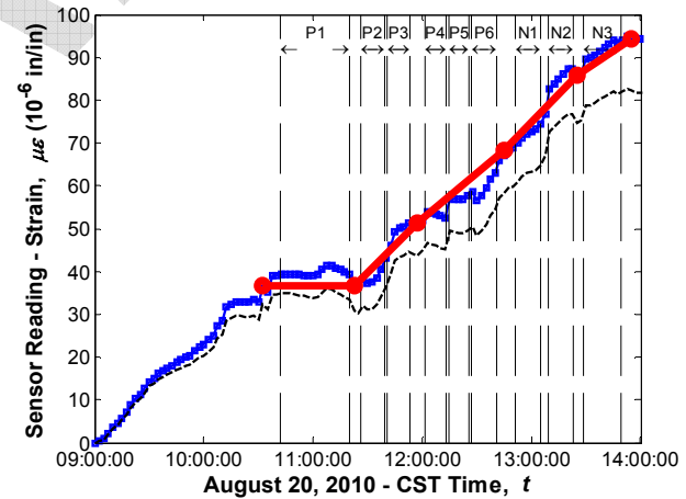
Sensor No. 53, Location G3S24, Support Top (Sisterbar)
