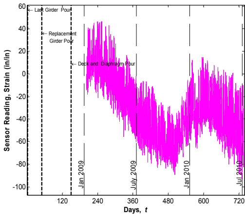
Sensor No. 41, Location G3S24, Support Bottom (Vibrating wire gauge)
