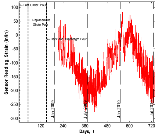
Sensor No. 2, Location G1S24, Support Bottom (Strandmeter)
