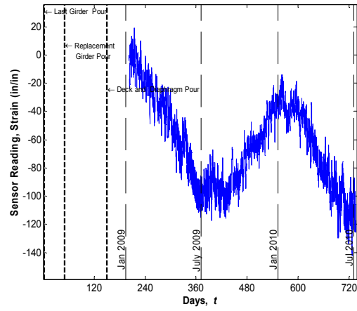
Sensor No. 95, Location G3S24, Midspan Deck (Sisterbar)
