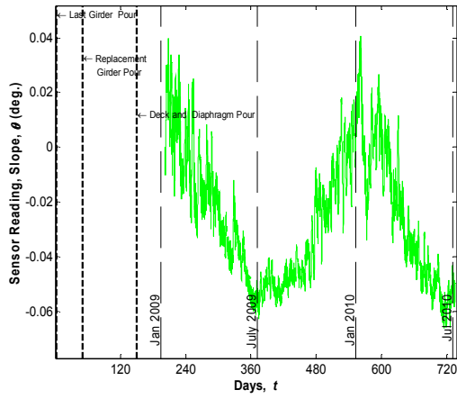
Sensor No. 55, Location G3S24, Support (Tiltmeter)
