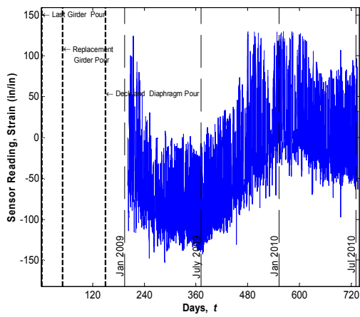
Sensor No. 47, Location G5S24, Support Top (Sisterbar)
