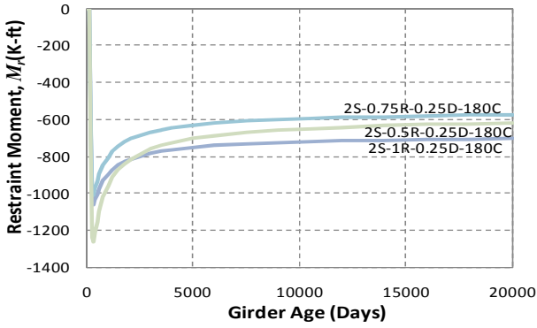
(a) Age = 180 days and I_{dia} = 0.25 \cdot I_g
