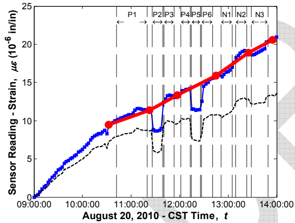
Sensor No. 81, Location G3S24, Midspan Top (Vibrating wire gauge)
