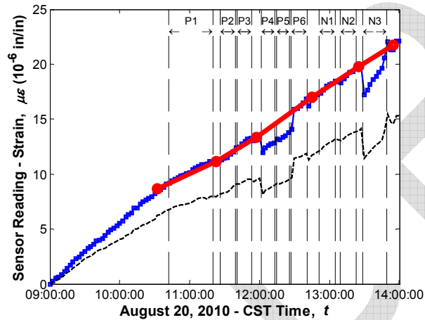
Sensor No. 18, Location G1S24, Support Middle (Vibrating wire gauge)
