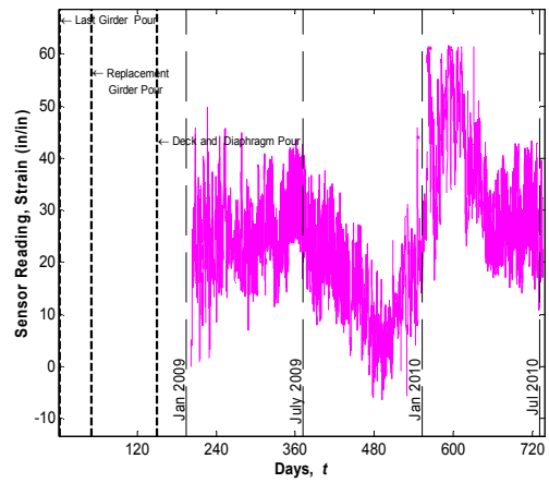
Sensor No. 17, Location G1S24, Support Top (Vibrating wire gauge)
