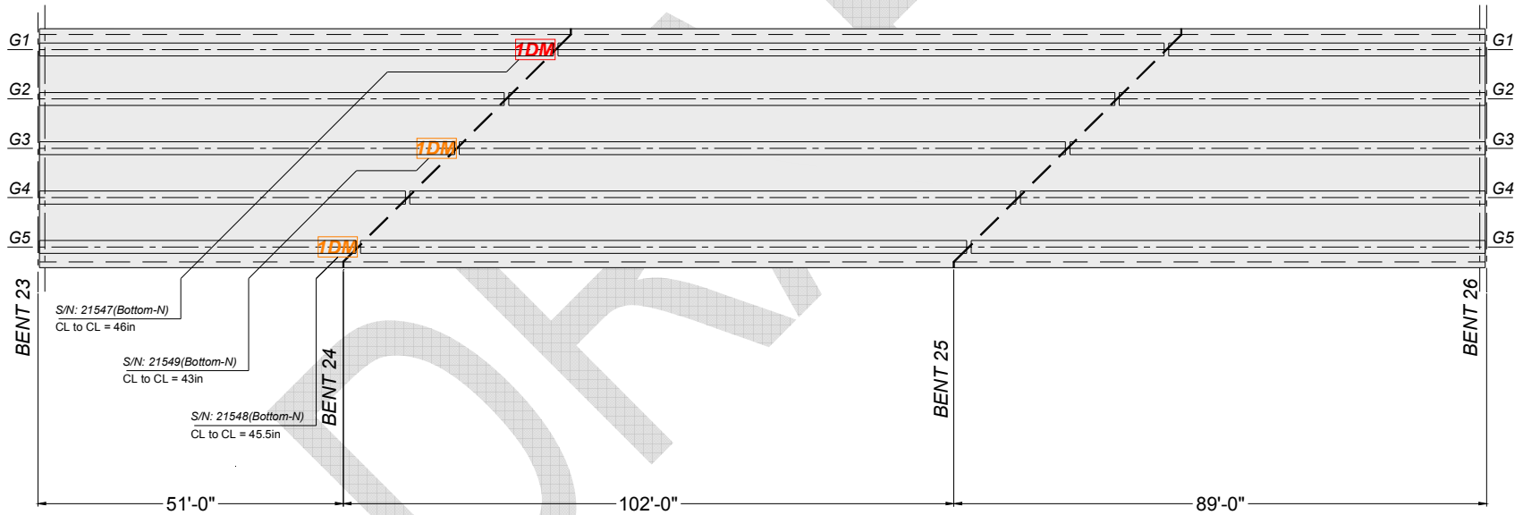
Figure A-16 Distribution of sensors on system multiplexers.
