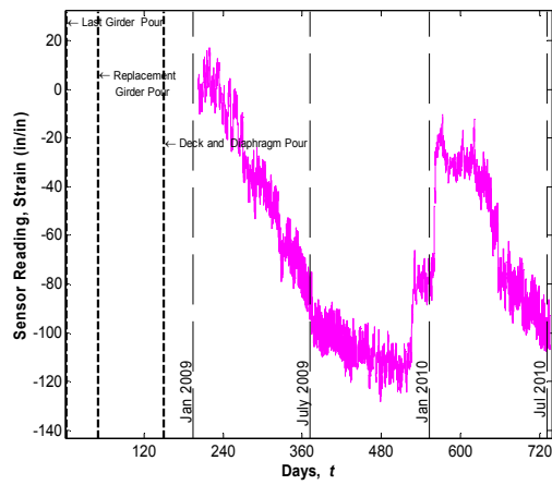
Sensor No. 42, Location G3S23, Support Top (Vibrating wire gauge)
