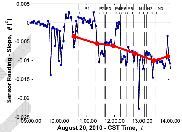
Sensor No. 56, Location G3S23, Support (Tiltmeter)
