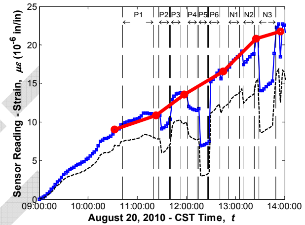
Sensor No. 21, Location G1S23, Support Middle (Vibrating wire gauge)
