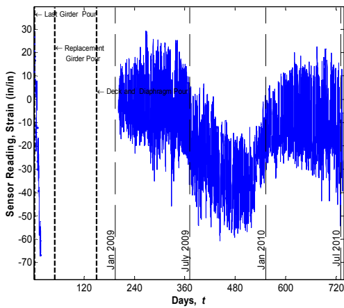
Sensor No. 92, Location G3S24, Midspan Bottom (Sisterbar)
