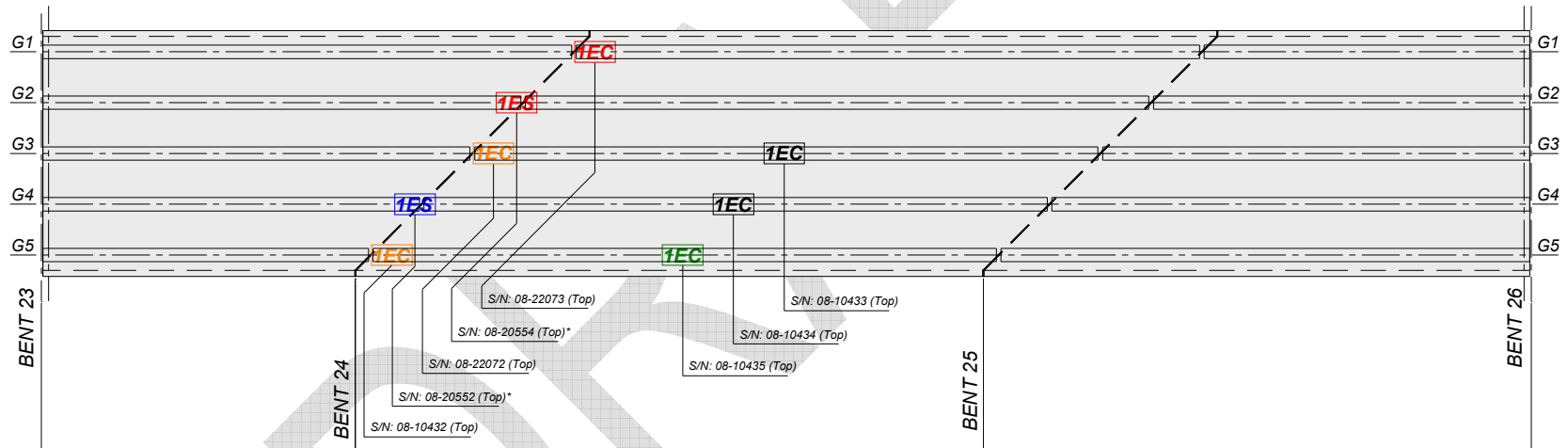
Figure A-14 Distribution of sensors on system multiplexers.
