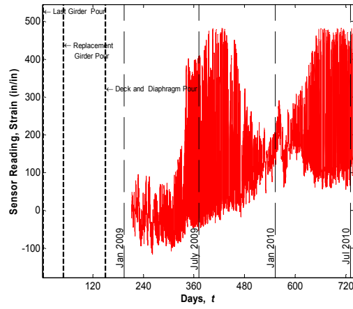
Sensor No. 50, Location G3S23, Support Bottom (Strandmeter)
