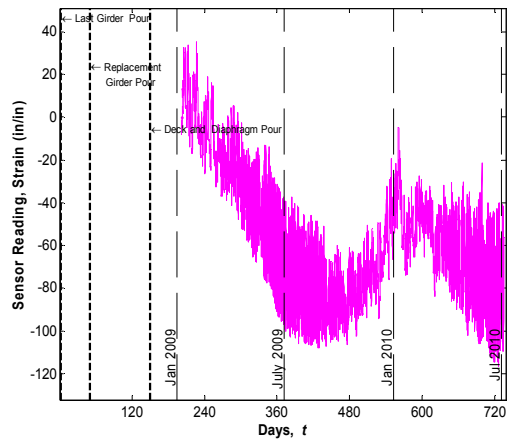
Sensor No. 65, Location G5S24, Midspan Top (Vibrating wire gauge)
