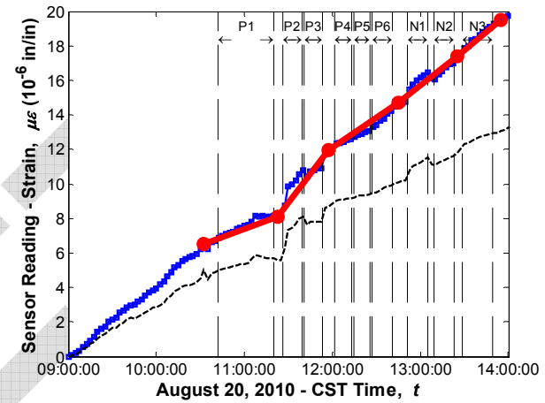
Sensor No. 39, Location G3S24, Support Top (Vibrating wire gauge)
