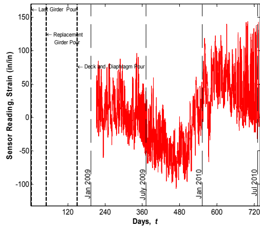
Sensor No. 46, Location G5S24, Support Bottom (Strandmeter)
