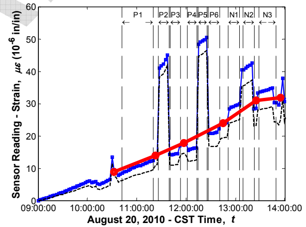
Sensor No. 94, Location G4S24, Midspan Bottom (Sisterbar)
