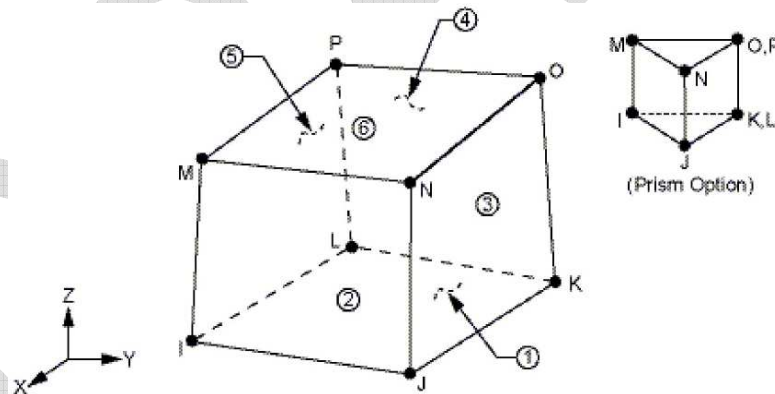
Figure E-1 Geometry, node and co-ordinate for SOLID5 element.
