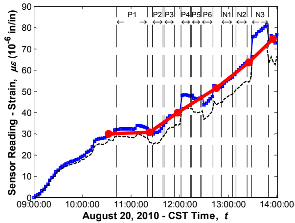
Sensor No. 5, Location G1S24, Support Top (Sisterbar)
