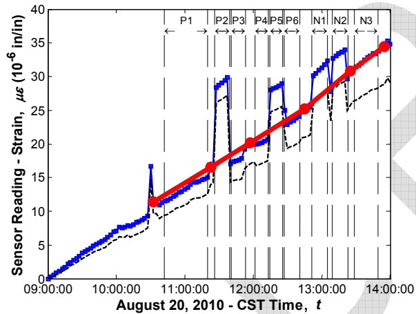
Sensor No. 85, Location G4S24, Midspan Middle (Vibrating wire gauge)
