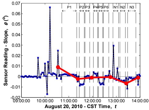
Sensor No. 55, Location G3S24, Support (Tiltmeter)
