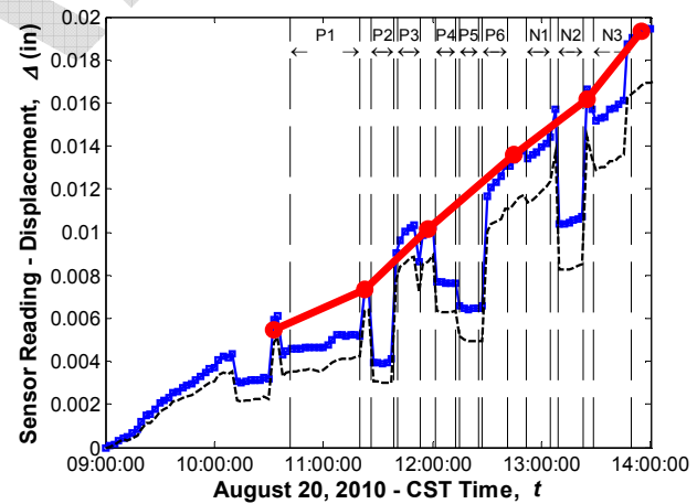
Sensor No. 58, Location G3, End Connection (Displacement meter)
