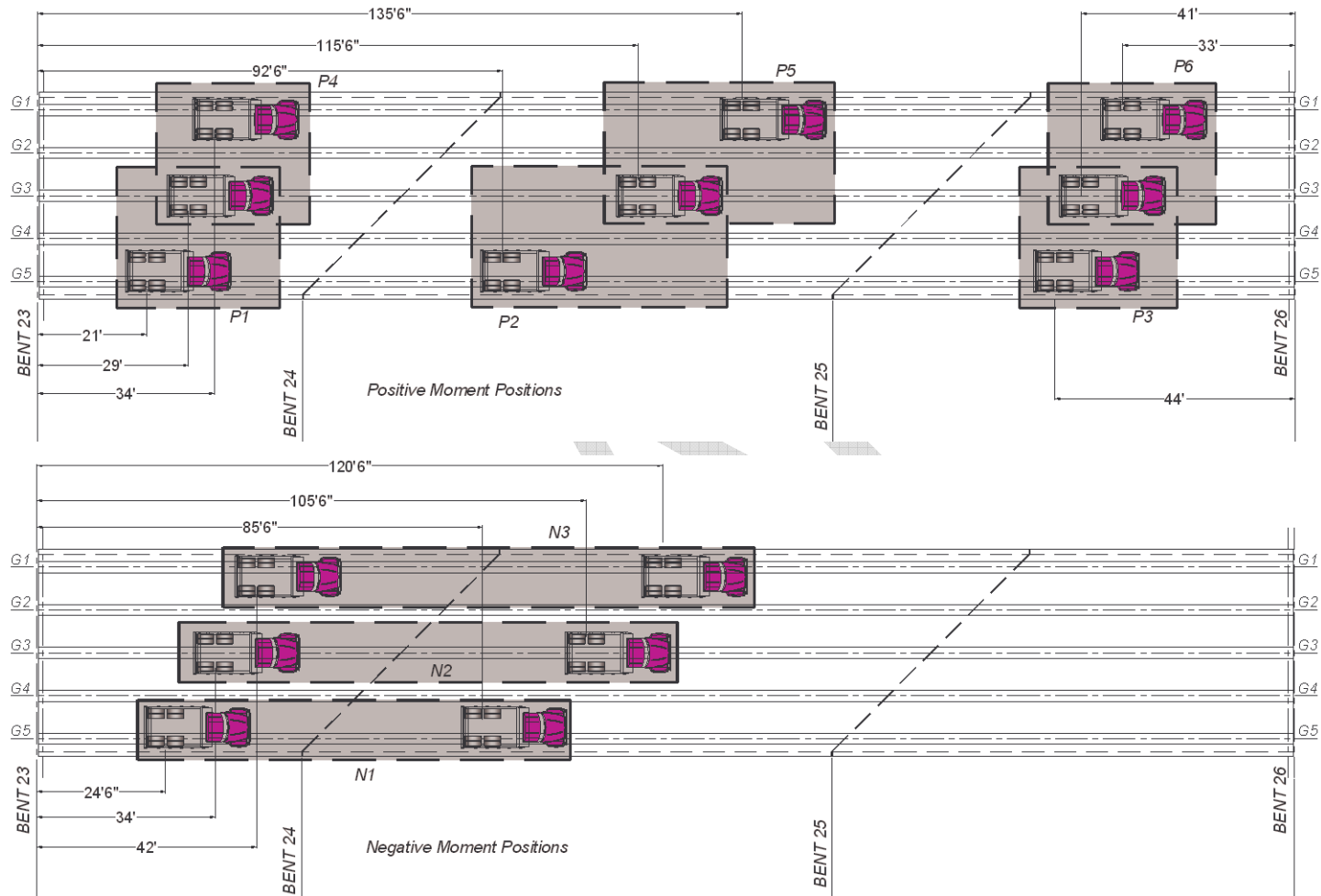
Figure 22 Load test truck positions (distance with reference to middle of rear drive axle – see Figure D-2).
