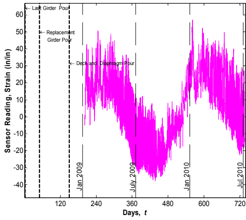
Sensor No. 33, Location G5S24, Support Top (Vibrating wire gauge)
