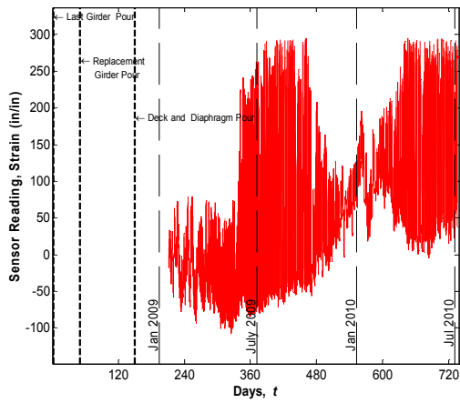
Sensor No. 51, Location G3S23, Support Bottom (Strandmeter)
