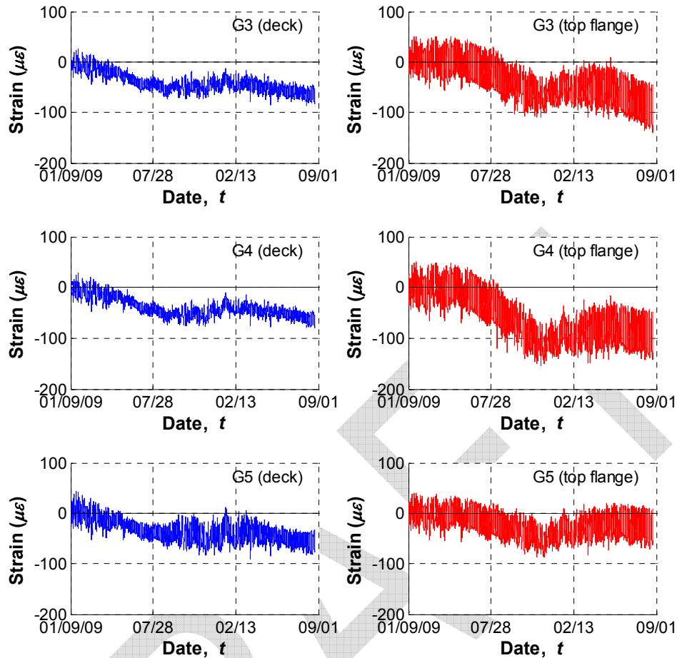
Figure 35 Strain records in deck and top flange at Girder G3, G4, and G5 locations.
