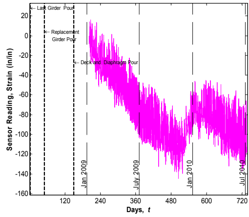
Sensor No. 85, Location G4S24, Midspan Middle (Vibrating wire gauge)
