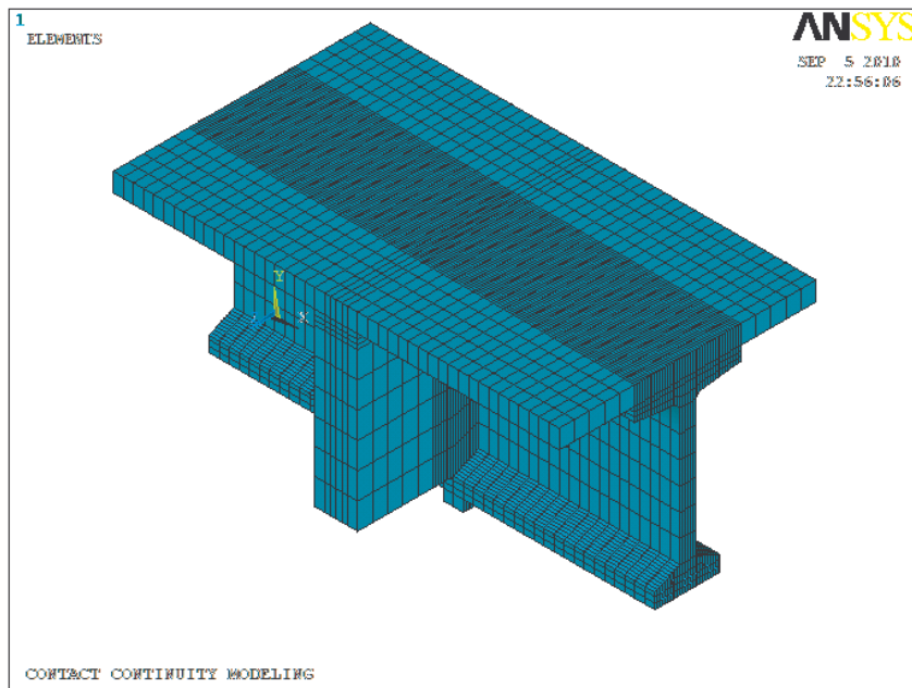
(b) finite element mesh
