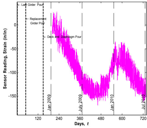
Sensor No. 43, Location G3S23, Support Middle (Vibrating wire gauge)
