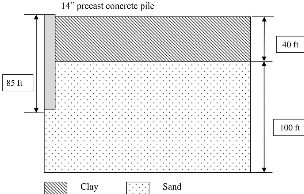
Figure 34 Soil profiles of Bayou Degleises Channel Bridge project
