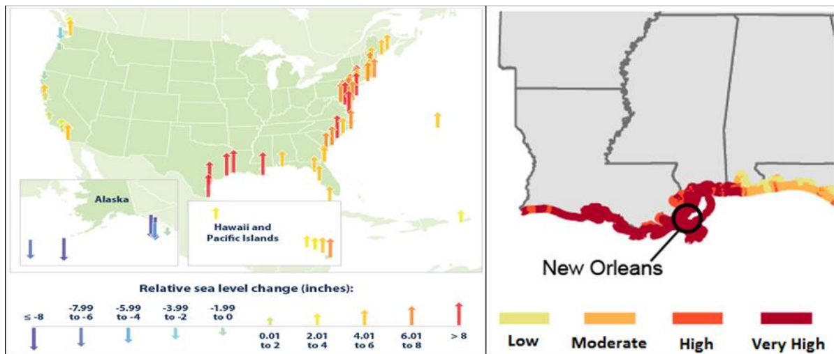
Figure 1 Left: Observed changes in sea level relative to land elevation in the United States between 1960 and 2014 (6). Right: The levels of risk sea level rise poses along Louisiana’s coastline, taking into consideration the susceptibility to change and adaptation measures (4).
