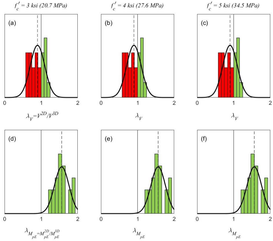
Figure 33. Histogram of straining action bias for different concrete compressive strengths, f'_c
